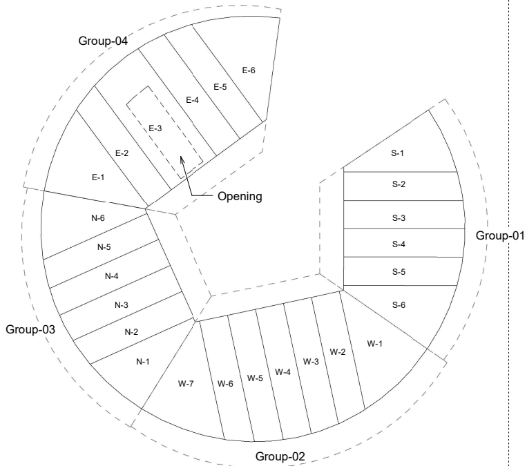
F6 Facade Flatten Plan View
