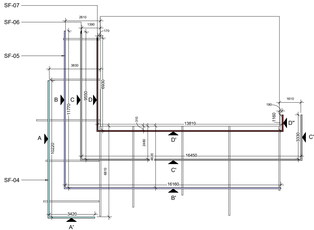
G1 Sub-Frame Detail
