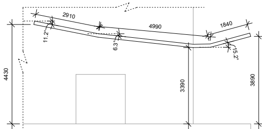
G1 Sub-Frame Detail
