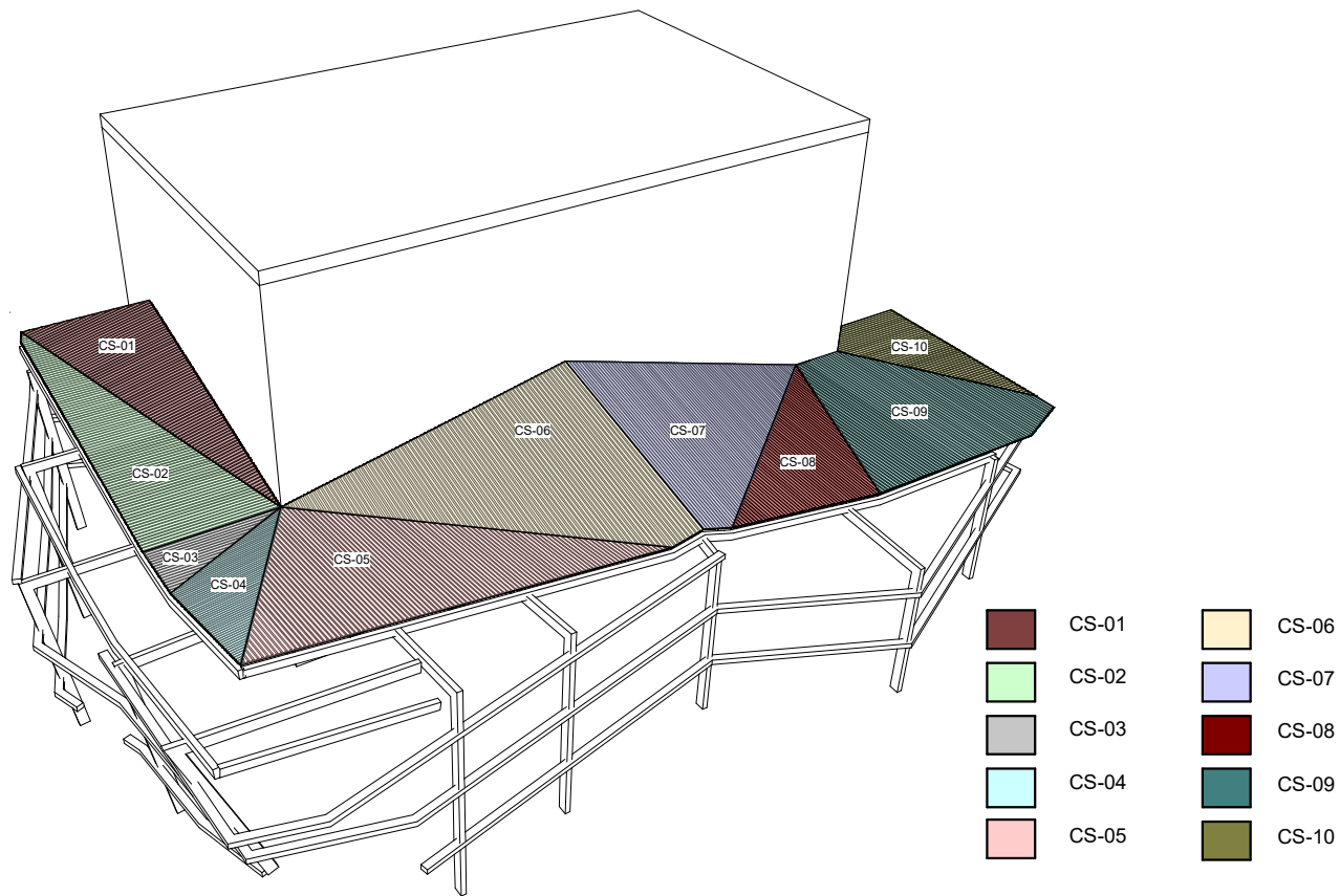
G1 Corrugated Sheet Detail
