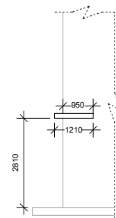
N9 SF-07 Section-DD'D" Detail
