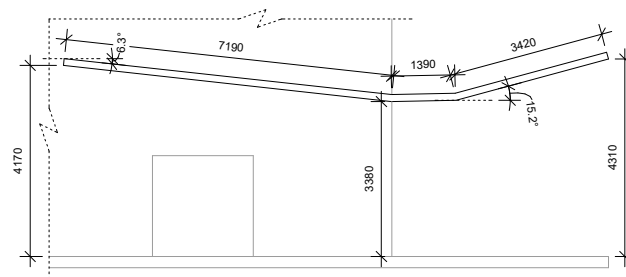
D9 SF-04 Section-AA' Detail
