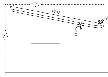
H9 SF-05 Section-BB' Detail
