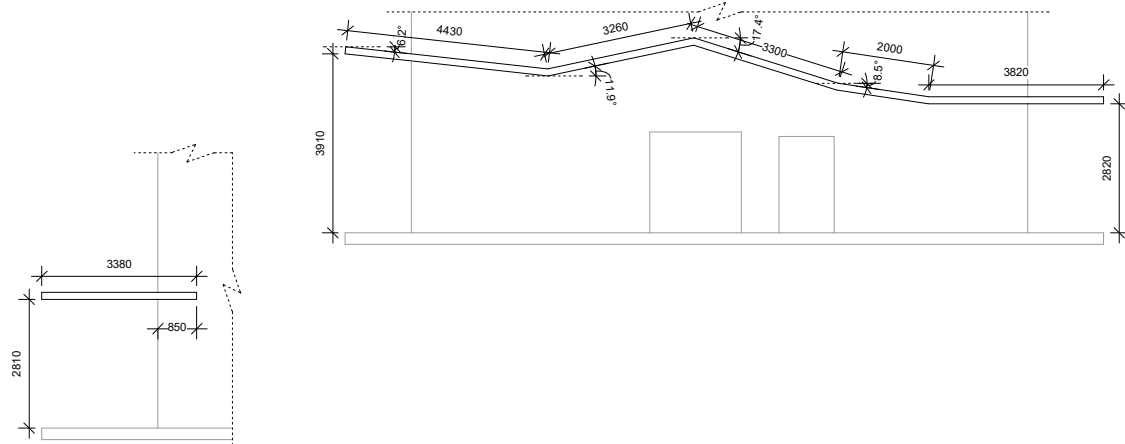
N1 SF-06 Section-CC'C" Detail
